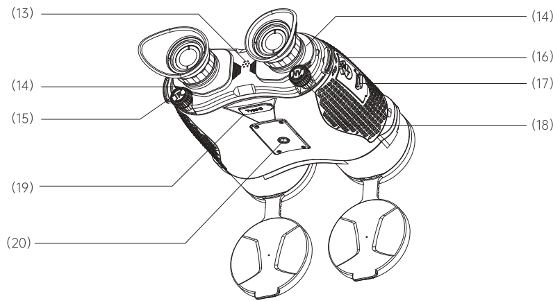
Figure 2 Rear View
